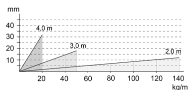
Deflection in mm at bracket spacing 2-4 m.
