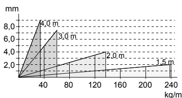
Deflection in mm at bracket spacing 1,5-4 m.
